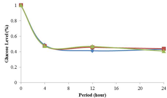
Figure 4. Comparison of Glucose Levels in Sample's Hydrolyzate Using S. cerevisiae (♦), F (■), and S (▲)
