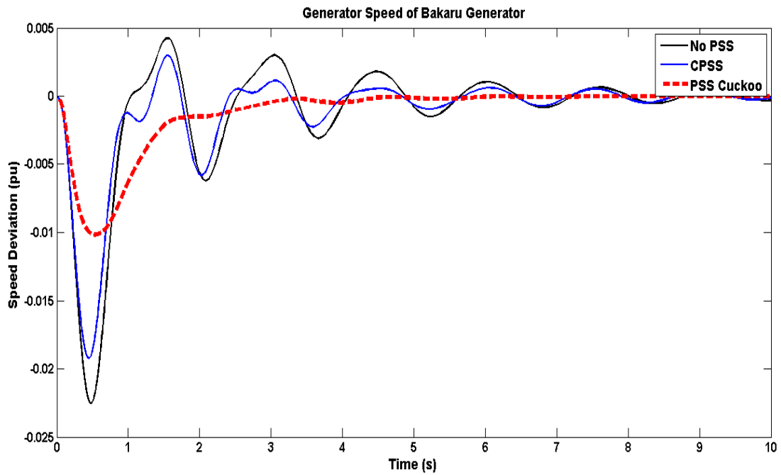
Figure 7. Speed Deviation ( \Delta\omega ) of the Bakaru Generator in the N-1 Condition
