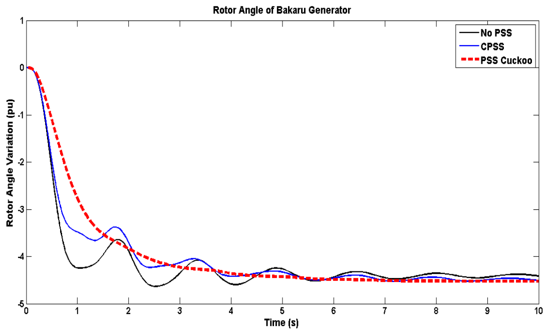
Figure 8. Rotor-Angle Variation of Bakaru Generator in the N-1 Condition
