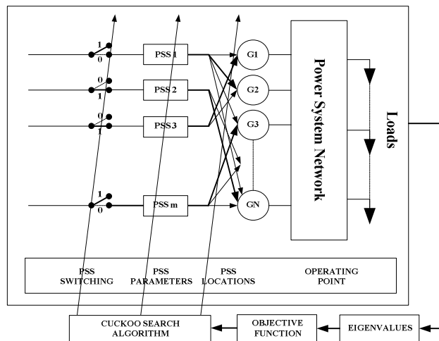
Figure 5. Representation-procedures Optimization
