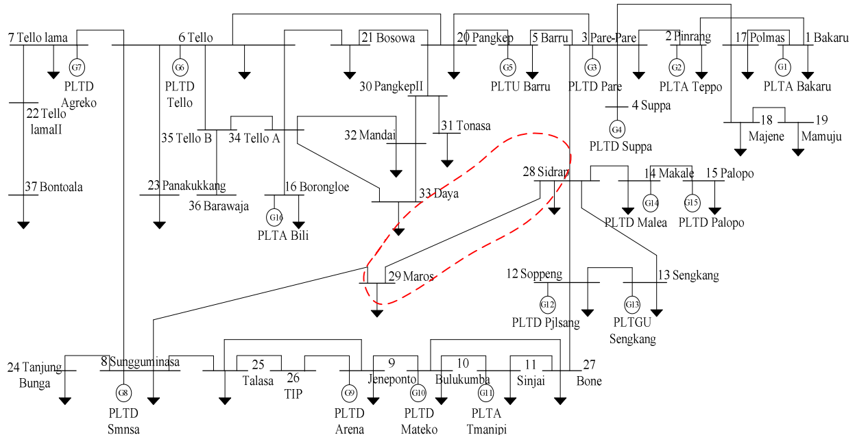
Figure 6. One-Line Diagram of the Sulselrabar Multimesin
