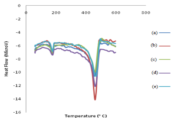
Figure 7. DTA Thermograms of the Samples Reinforced with Different Quantities of Calcined Zeolite (a) PP, (b) 0 wt%, (c) 2 wt%, (d) 4 wt%, (e) 6 wt%
