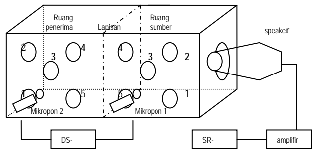
Gambar 1. Kotak Pengujian Sound Transmission Loss (STL)
