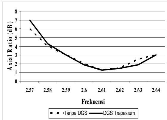
Gambar 4. Hasil simulasi axial ratio
