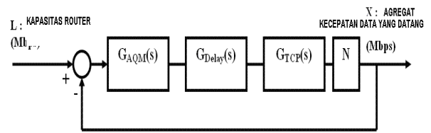
Gambar 2. Diagram Blok Sistem Kendali Kongesti
