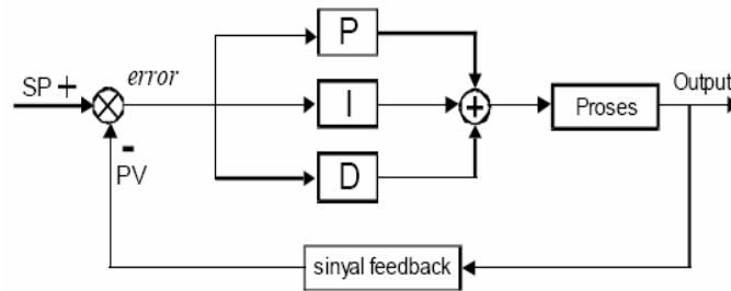
Gambar 1. Kendali PID [5]
