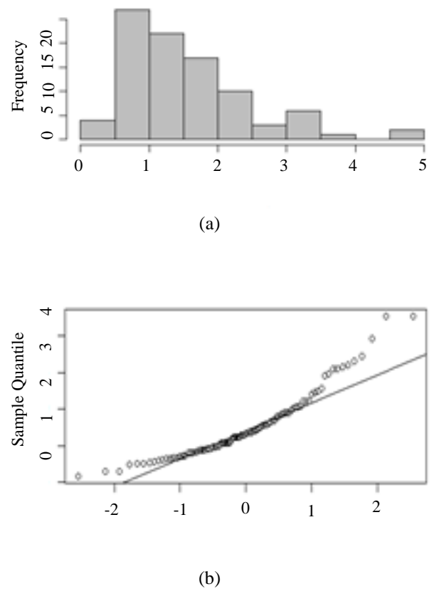
Figure 1. (a) Histogram and (b) normal QQ plot for birth weight data
